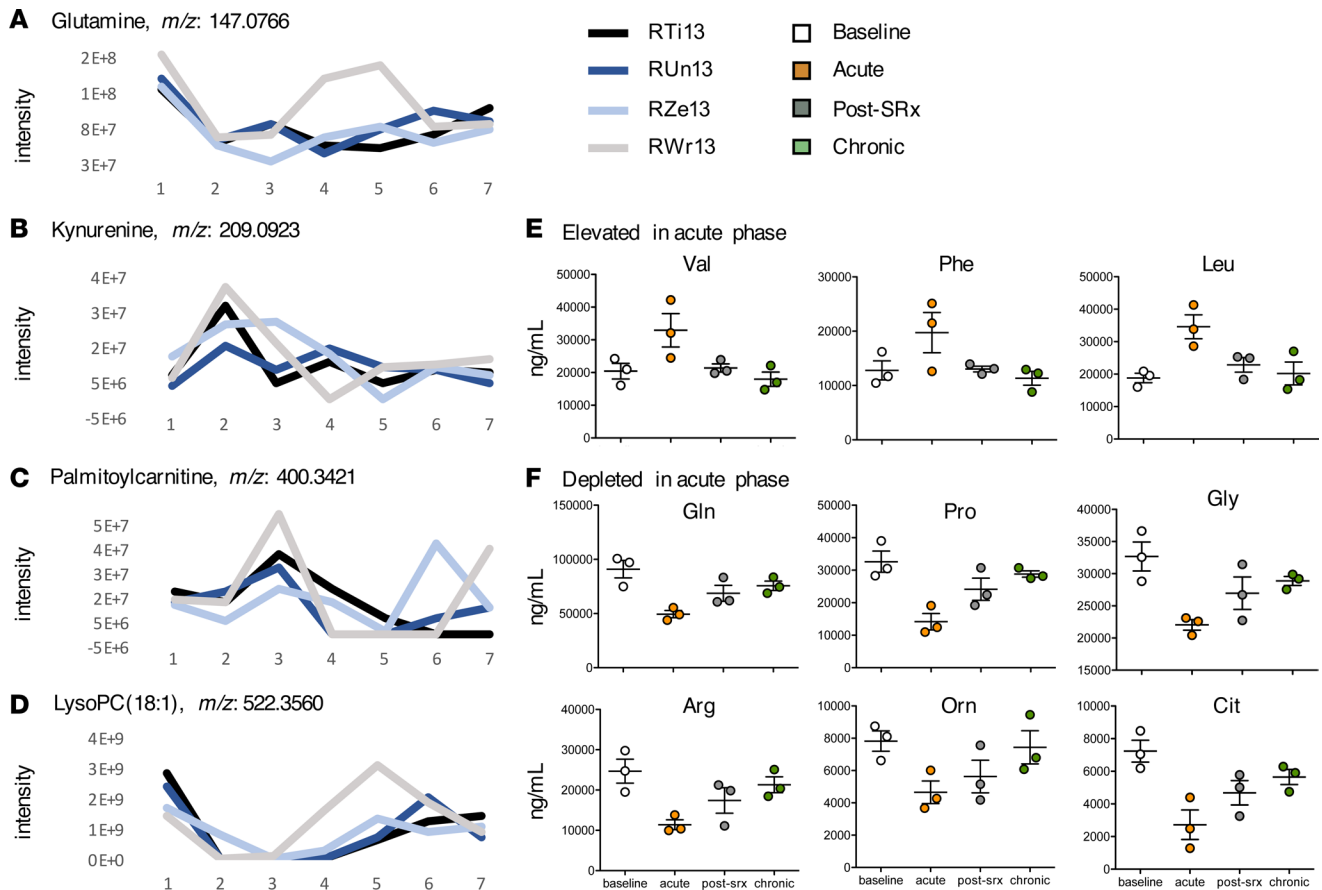
Figure 4. Temporal fluctuations observed in amines, lipids, and carnitines. (A–D) Relative intensity data (LC-MS) across all 7 TPs and all 4 animals for 4 metabolites confirmed by LC-MS/MS (metabolite identification level 2a) significantly altered during infection; from top to bottom, metabolites shown are the M+H adducts of glutamine (A), kynurenine (B), palmitoylcarnitine (C), and lysoPC (18:1) (D). (E and F) Quantitative plasma concentration data at each clinical phase for significantly altered amino acids with a peak (E) or nadir (F) during the acute phase. Each of the amino acids shown demonstrated a statistically significant difference in plasma concentration across phases (repeat-measures ANOVA, P < 0.05 , N = 3 ) except for Phe, which had a borderline P value of 0.054. Error bars indicate mean \pm SEM per phase. Colors indicate phase: baseline (white), acute (orange), post-subRx (gray), and chronic (green). Orn ornithine; Cit, citrulline.
