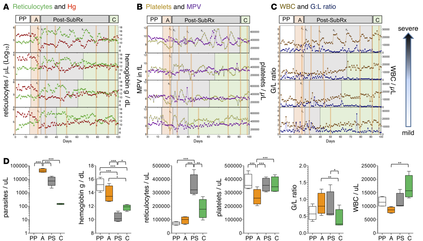
Figure 2. Dynamic hematological changes across longitudinal phases of infection with P. coatneyi in rhesus macaques. (A–C) Longitudinal hematological parameters from all animals as measured daily by complete blood counts from capillary blood draws. Vertical orange lines denote TP collections. Rx denotes timing of subcurative treatment with artemether. (A) Hematopoietic measurements: reticulocytes expressed in number/ \mu\text{L} (green) against hemoglobin (Hb) expressed in grams/deciliter (g/dl) (red). (B) Platelet indices: Platelet counts expressed in number/ \mu\text{L} (yellow) against mean platelet volume (MPV) expressed in femtoliters (fl) (purple). (C) Leukocyte indices: white blood cell (WBC) count expressed in number/ \mu\text{L} (orange) against granulocyte/lymphocyte (G/L) ratios (blue). (D) Hematological parameters per clinical phases (mean \pm range, N = 4 ). * P < 0.05 ; ** P < 0.01 ; *** P < 0.001 by repeated-measures ANOVA with Bonferroni's correction. PP, pre-patent; A, acute; PS, post-subcurative treatment; C, chronic.
