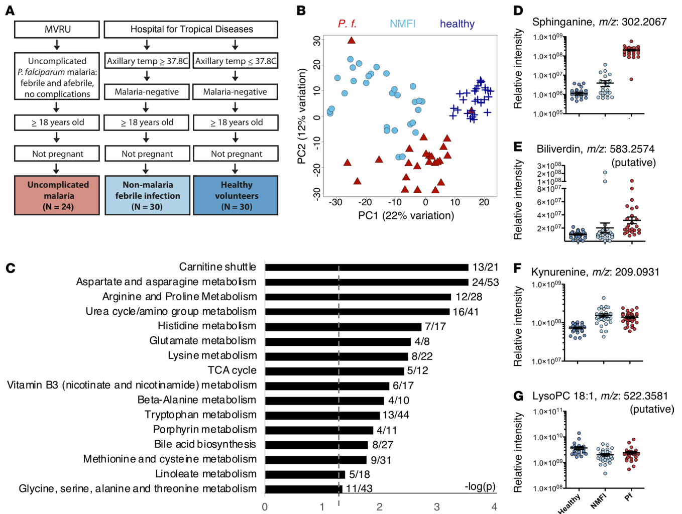
Figure 7. Human malaria exhibits both common and distinct metabolite perturbations as compared with other febrile illnesses. (A) Criteria for enrollment in this study. (B) Unsupervised, global PCA plot of LC-MS features with data points representing individuals, shape and color-coded by disease categories: P. falciparum ( P. f. , red triangles), NMFI (light blue circles), and healthy (dark blue crosses). (C) Metabolic pathways significantly enriched in malaria compared with non-malaria using untargeted data (metabolic pathway analysis using mummichog , P < 0.05 ). The number of genes in the data set and in the pathway are shown. (D and E) Metabolites (from LC-MS) significantly altered (repeat-measures ANOVA with Benjamini-Hochberg FDR correction, P < 0.05 ) specifically in malaria cases include sphinganine (confirmed by LC-MS/MS; metabolite identification level 2a) and biliverdin (putative; metabolite identification level 2b). (F and G) Metabolites (from LC-MS) significantly altered (FDR-corrected P < 0.05 ) in both malaria and NMFI cases include kynurenine (confirmed by LC-MS/MS; metabolite identification level 2a) and lysoPC 18:1 (putative; metabolite identification level 2b).
