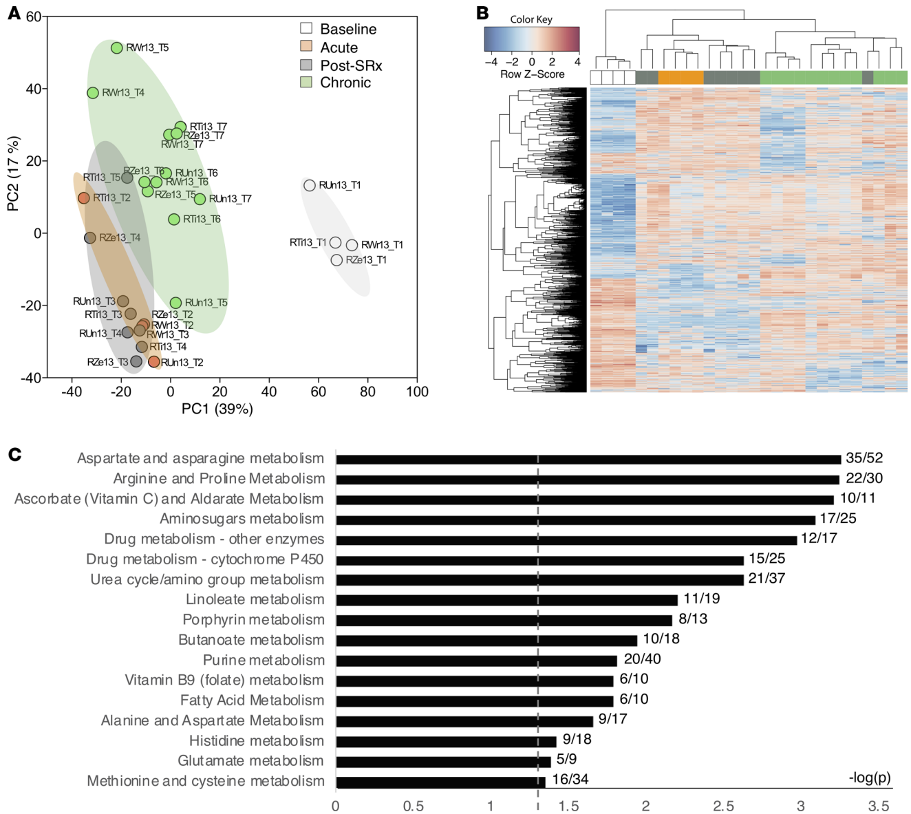
Figure 3. Significant perturbations in plasma metabolites occur during disease progression in rhesus macaques. (A) Unsupervised, global PCA plot of 5,712 metabolite features. Each dot represents an individual TP for each animal. Color-coded ellipses indicate clinical phases. (B) HCA of metabolite features significantly changed across phases (each row is one metabolite feature, each column is one sample from a given TP and animal), with statistical significance determined using repeat-measures ANOVA with Benjamini-Hochberg FDR correction, P < 0.05 , N = 4 . (C) Significantly enriched metabolic pathways based on untargeted LC-MS data (pathway enrichment using mummichog , P < 0.05 ).
