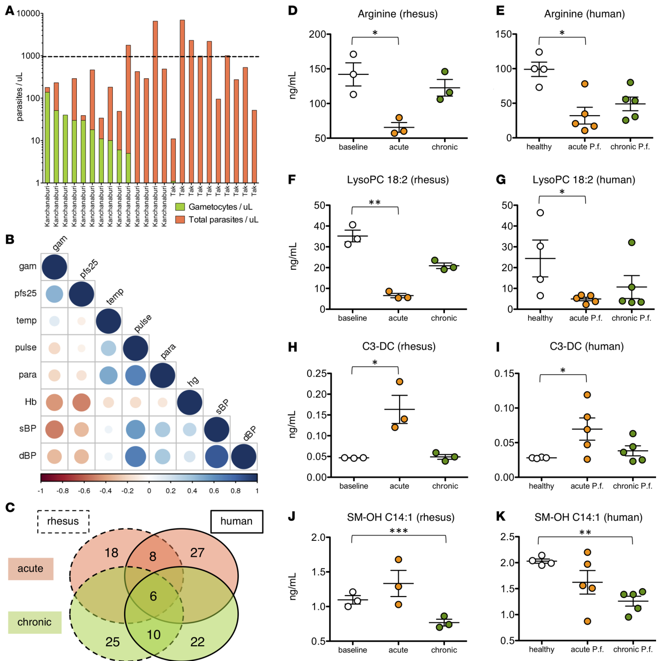
Figure 8. Human malaria infections recapitulate acute and chronic-like metabolic profiles. (A) Parasite asexual- and sexual-stage distribution in Thai P. falciparum cases by microscopy. (B) Spearman's correlation of metadata for P. falciparum cases. Blue, positive correlation. Red, negative correlation. Abbreviations are as follows: gam, gametocytes per microliter by microscopy; pfs25, gametocyte gene Pfs25 marker expression by RT-PCR; temp, body temperature; pulse, heart rate/pulse in beats per minute; para, parasites per microliter by microscopy; hg, hemoglobin level; sBP, systolic blood pressure; dBP, diastolic blood pressure. (C) Venn diagram of metabolites confirmed by targeted MS/MS that significantly differ between acute and chronic malaria in rhesus macaques and humans ( P < 0.05 by 2-tailed t test). Orange indicates acute malaria, and green indicates chronic malaria. (D–K) Dot plots of the concentration of metabolites in plasma in rhesus macaques (baseline, acute, chronic) and in humans (healthy, acute Pf. , chronic Pf. ), showing mean and SEM and including arginine (D and E), lysoPC 18:2 (F and G), C3-DC (H and I), and SM-OH C14:1 (J and K). * P < 0.05 ; ** P < 0.01 ; *** P < 0.001 by 2-tailed t test.
